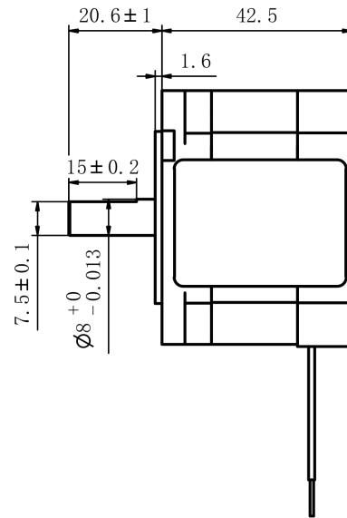
Mechanical View 2
