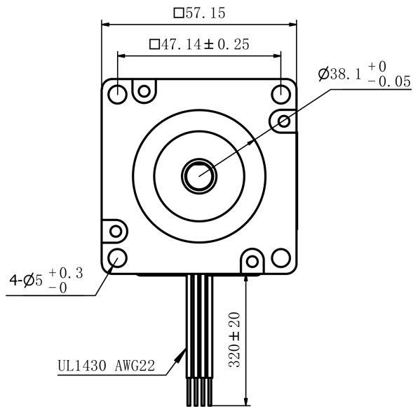
Mechanical View 1
