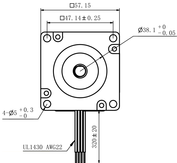
Mechanical View 1
