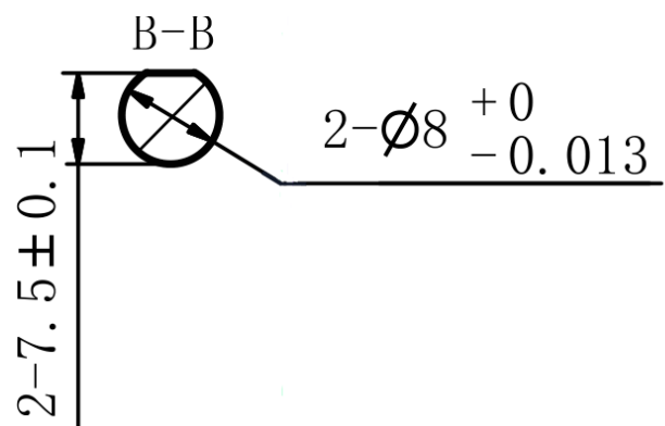
Mechanical View 5
