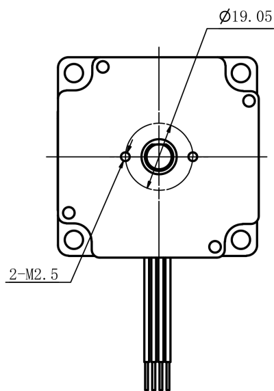
Mechanical View 3
