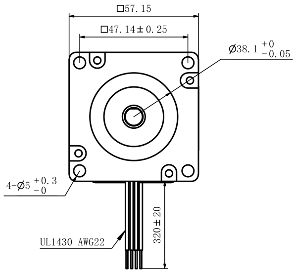
Mechanical View 1
