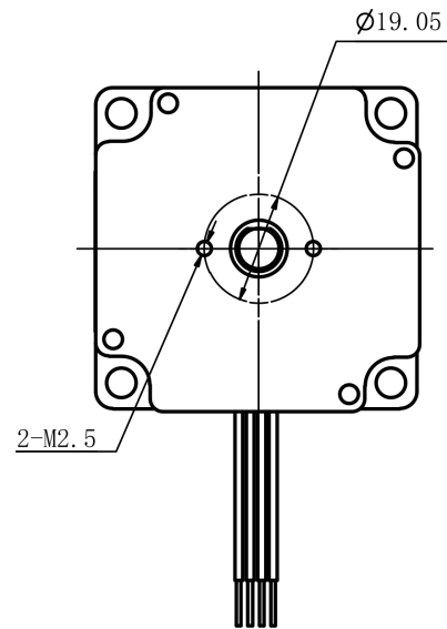
Mechanical View 2
