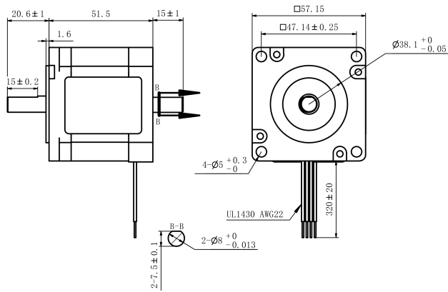
Mechanical View 1
