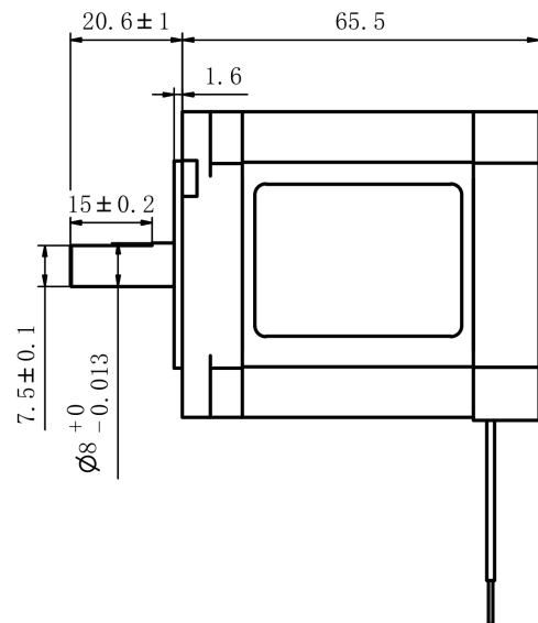
Mechanical View 2
