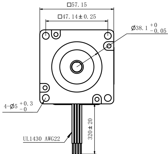
Mechanical View 1
