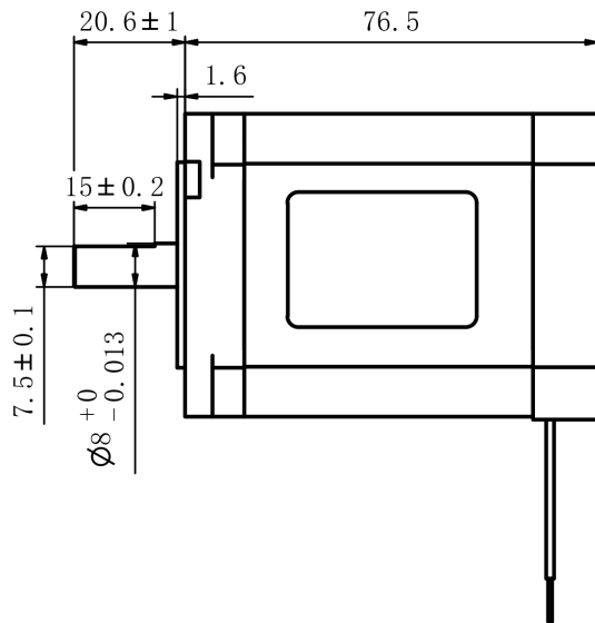
Mechanical View 1
