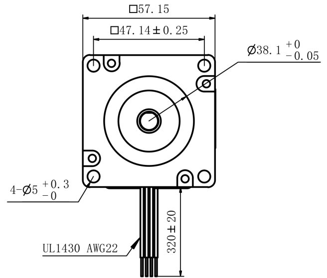
Mechanical View 2
