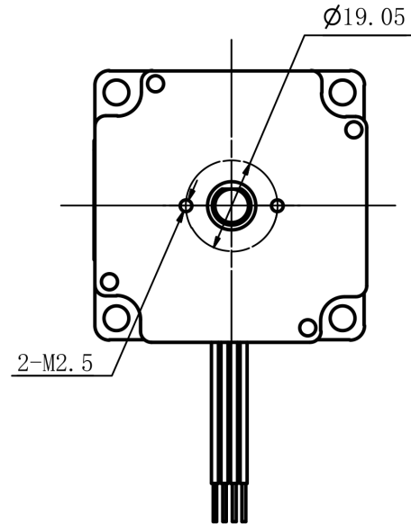
Mechanical View 2
