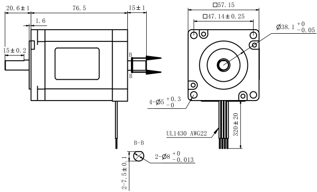
Mechanical View 1
