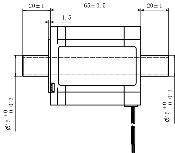
Mechanical View 1
