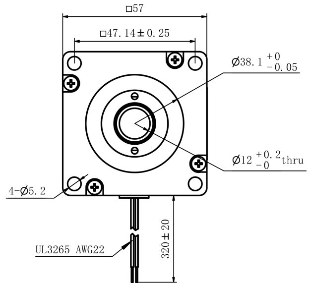
Mechanical View 2
