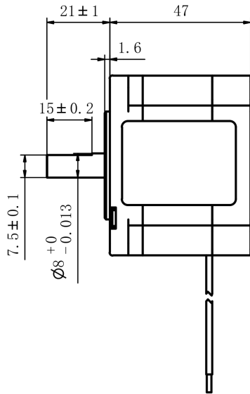
Mechanical View 1
