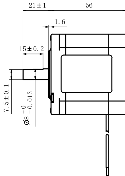
Mechanical View 1
