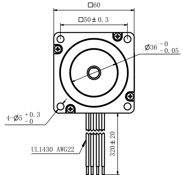
Mechanical View 2
