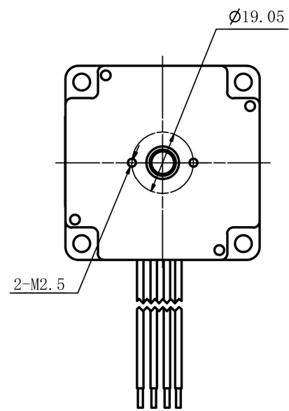
Mechanical View 2
