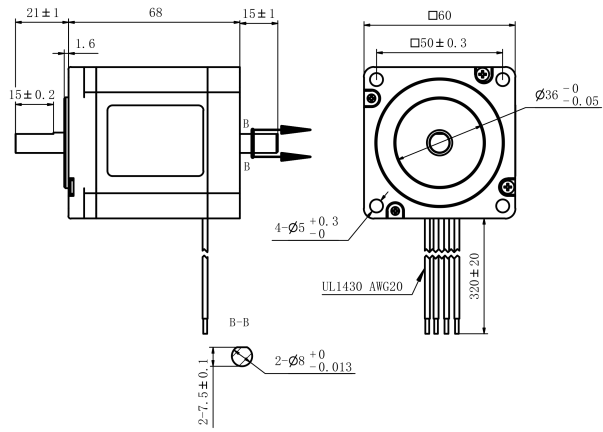
Mechanical View 1
