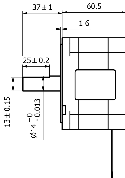
Mechanical View 1
