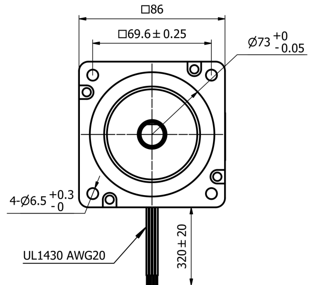
Mechanical View 2
