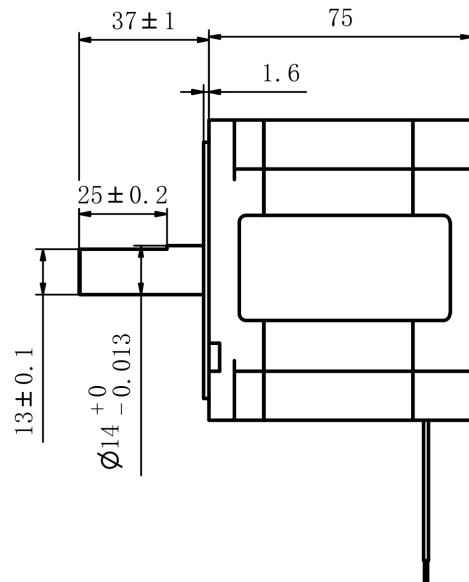
Mechanical View 2
