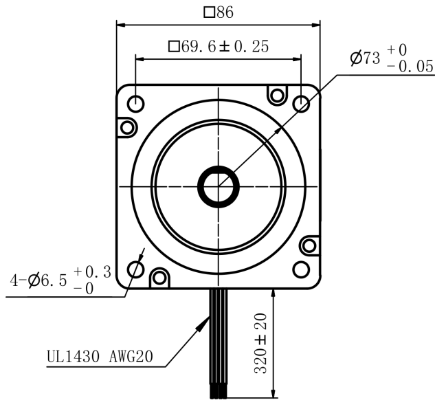
Mechanical View 1
