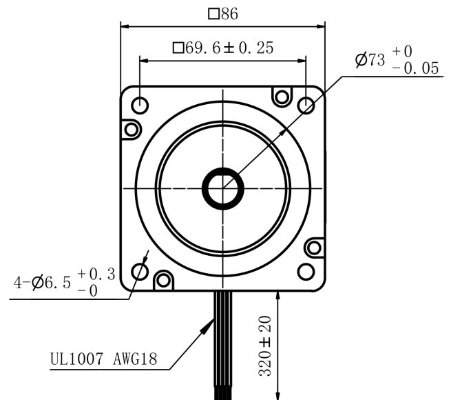
Mechanical View 2
