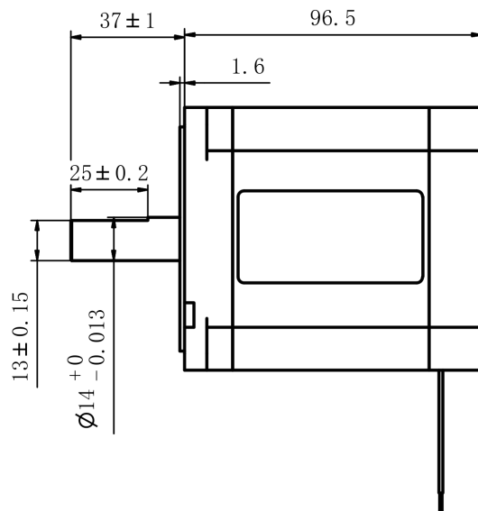
Mechanical View 1
