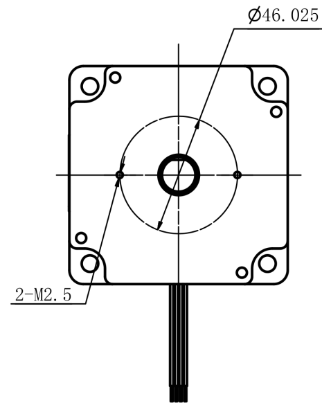
Mechanical View 2
