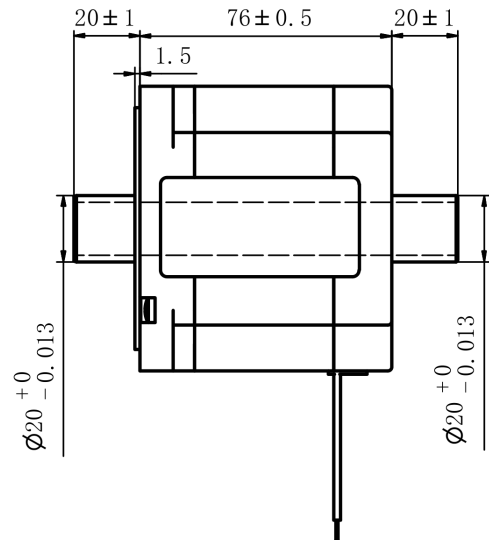
Mechanical View 2
