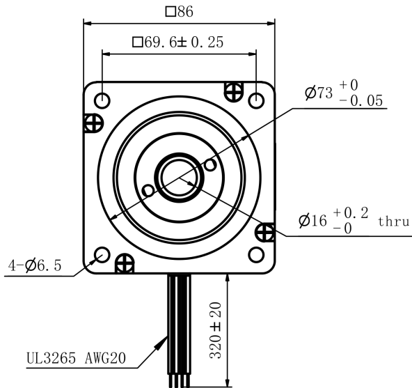
Mechanical View 1
